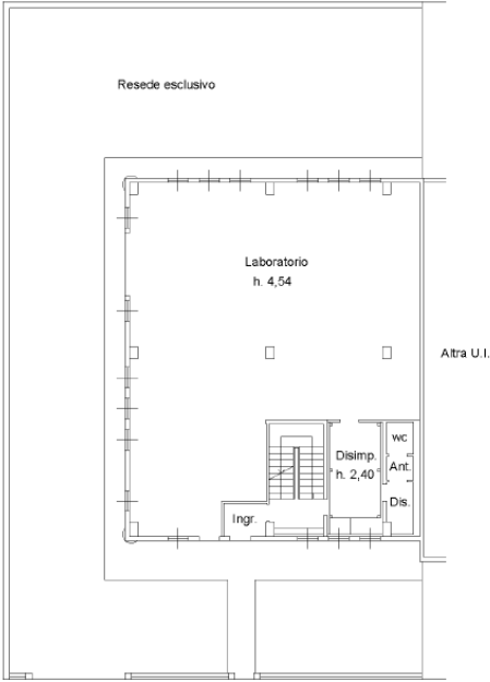
PIANO TERRA
